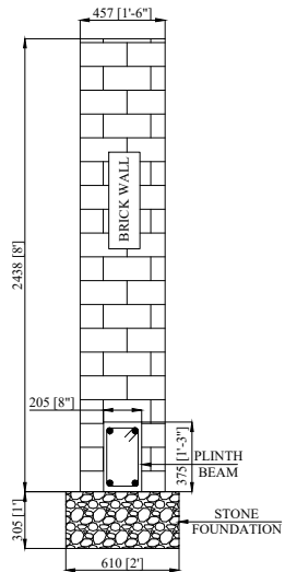
CROSS SECTION
